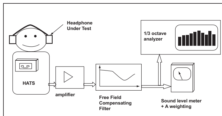
Fig. 5: Test Configuration for British Standard BS EN 50332
