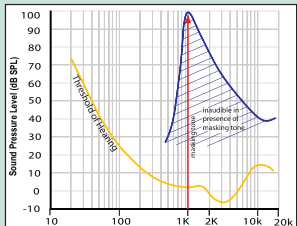
Fig. 3: A masking curve is used to eliminate 'unheard' sounds
