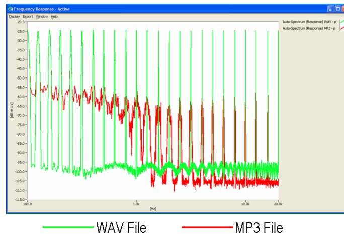
Fig 4: Noise floor of MP3 and WAV files.
