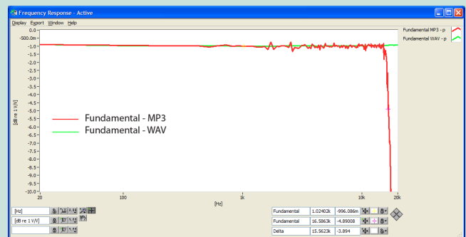
Fig. 2: High frequency cut-off of an MP3 file compared to a WAV file
