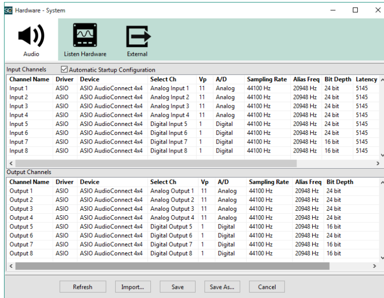
Figure 2-1: Windows Hardware Editor
