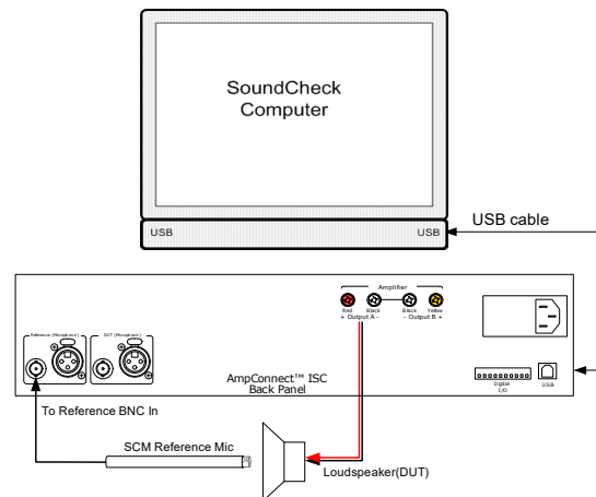
Figure 4: Complete Test Wiring
