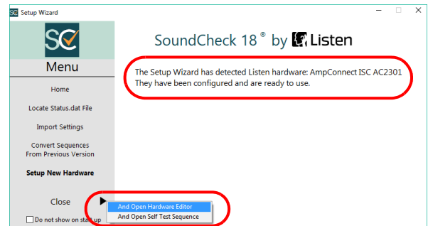
Figure 1: Setup Wizard
